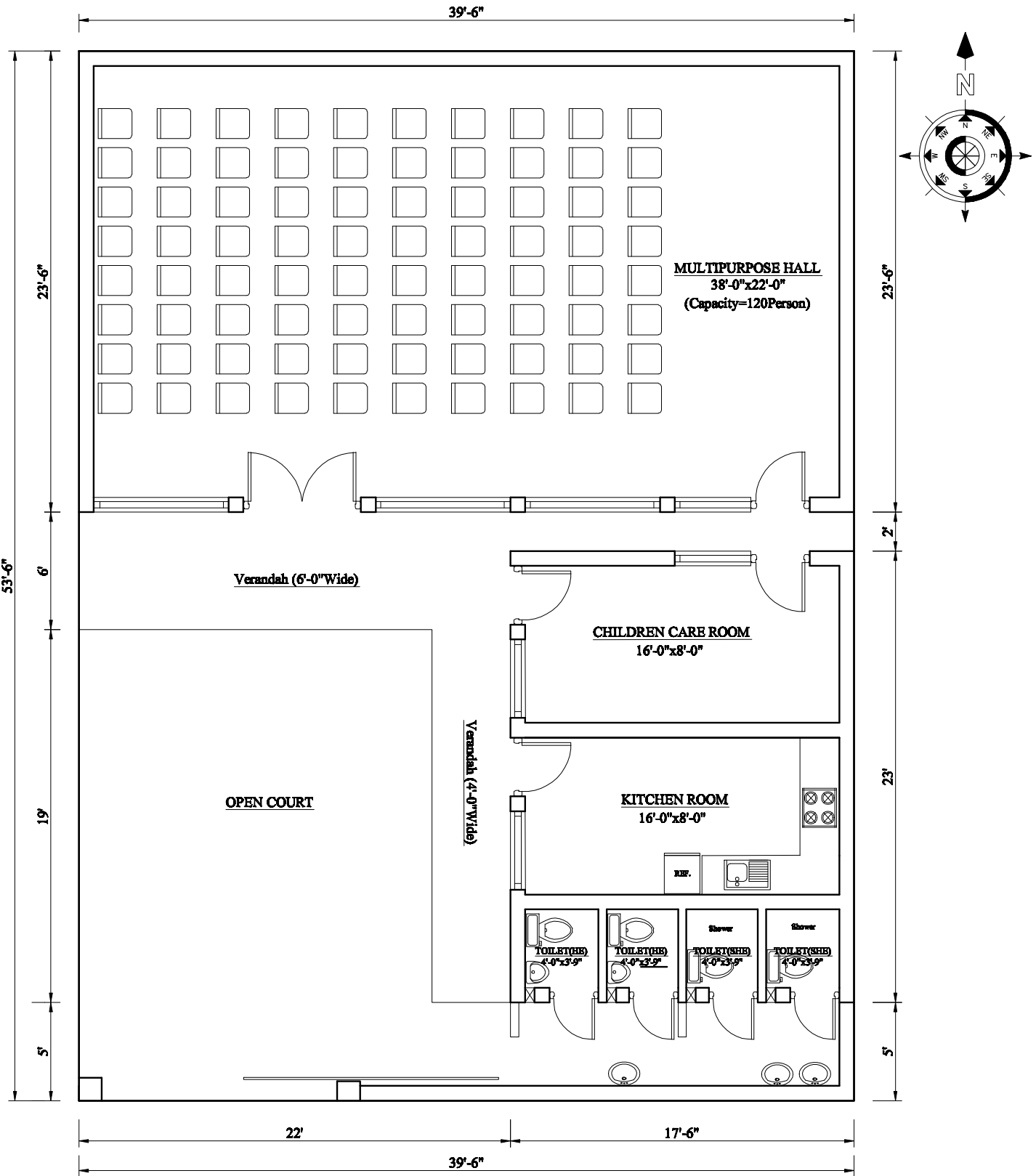
GROUND FLOOR PLAN Area: (1575.00 Square ft.) Land Area: 2113.25 Sq. ft
